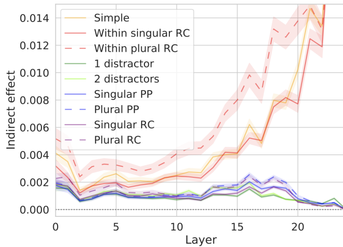
Figure 12 GPT-2 Medium shows a dissociation between local (shown in red/yellow) and non-local (shown in purple/green) agreement. Figure from Finlayson et al. (2021: 1834-1835) .
